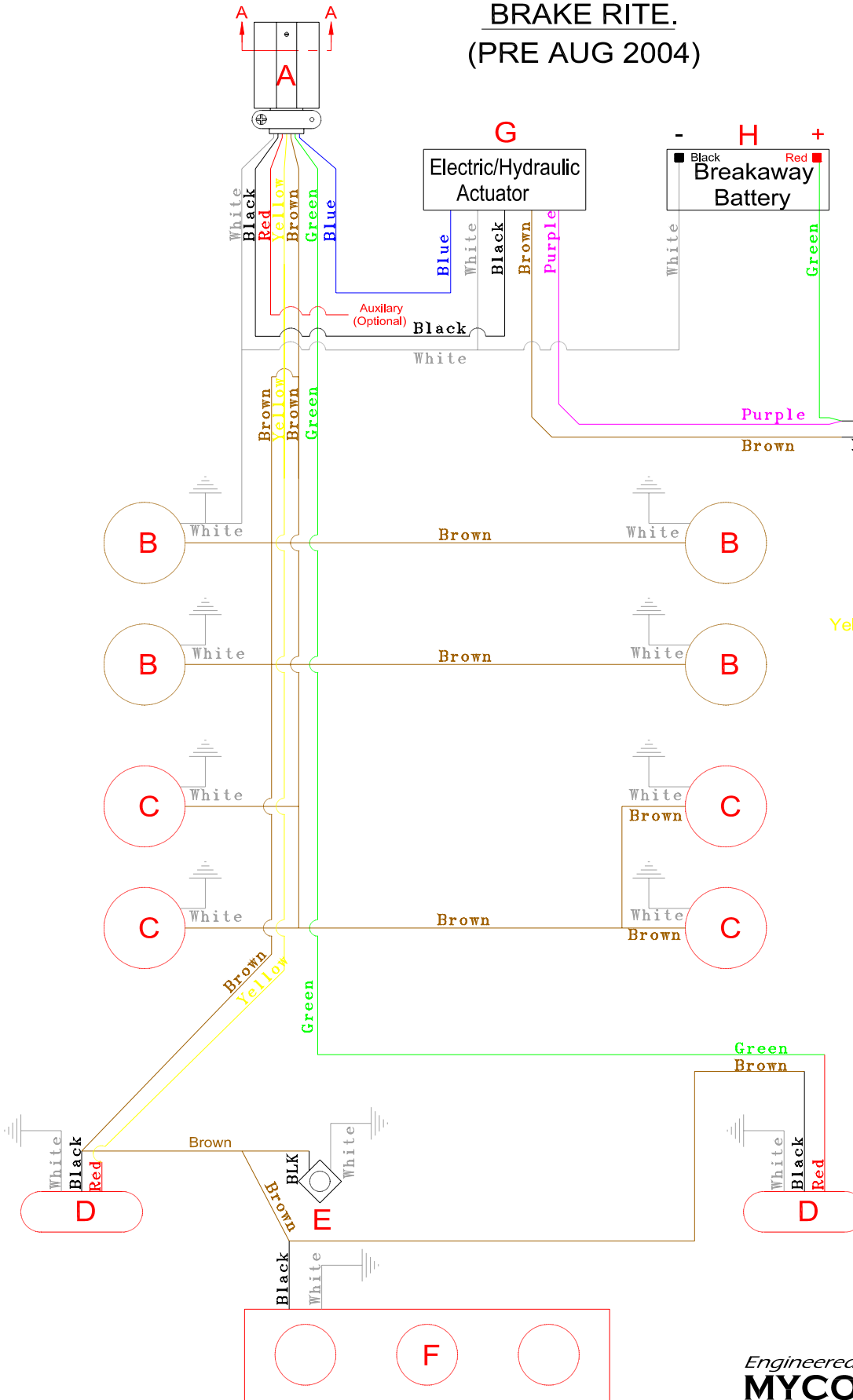
Plug, 7 Blade, Wiring Diagram.
