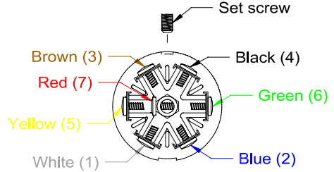
Plug, 7 Blade, Wiring Diagram.
