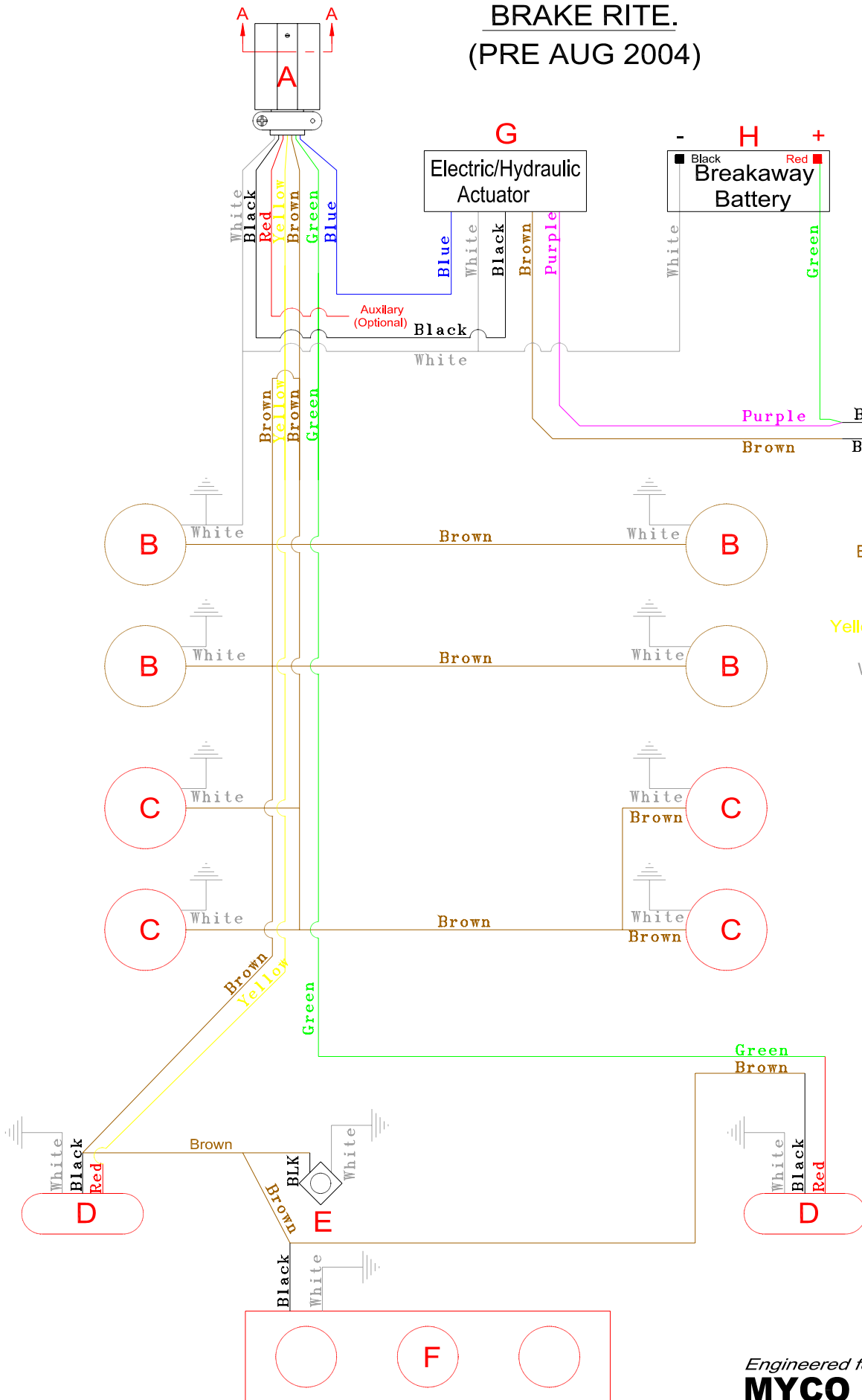
Plug, 7 Blade, Wiring Diagram.
