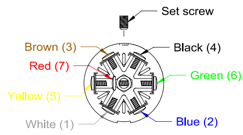
Plug, 7 Blade, Wiring Diagram.
