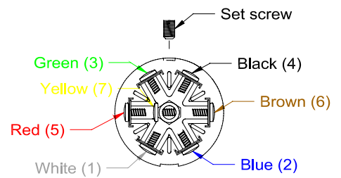
Plug, 7 Blade, Wiring Diagram.
